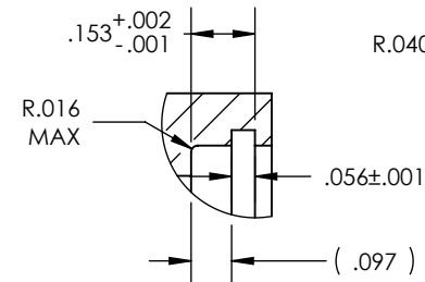
DETAIL D SCALE 2 : 1
