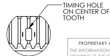
DETAIL F SCALE 1 : 1
